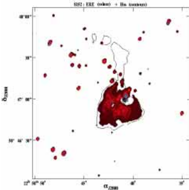
Fig. 7. ERE distribution (colors) and H \alpha emission (solid contours) in Sh 152
