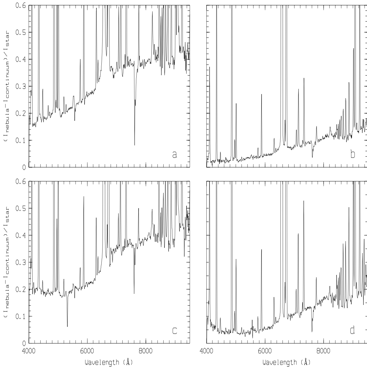
Fig. 3. Division of the nebula spectra corrected for atomic continuum emission by the spectrum of the exciting star, for regions 1 (a), 2 (b), 3 (c) and 4 (d) (see Fig. 1)
