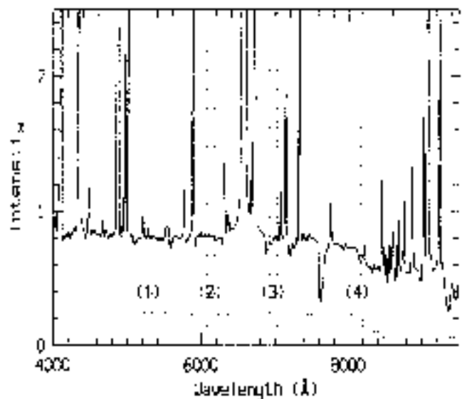
Fig. 2. Dereddened spectrum of region 1 of Sh 152; the theoretical atomic continuum spectrum is superimposed in dotted line (intensity in 10^{-6} \text{ erg cm}^{-2} \text{ s}^{-1} \text{ \AA}^{-1} \text{ sr}^{-1} ). Vertical dotted lines indicate the bandpasses (1) to (4) of the filters used for narrow-band imaging of Sh 152.
